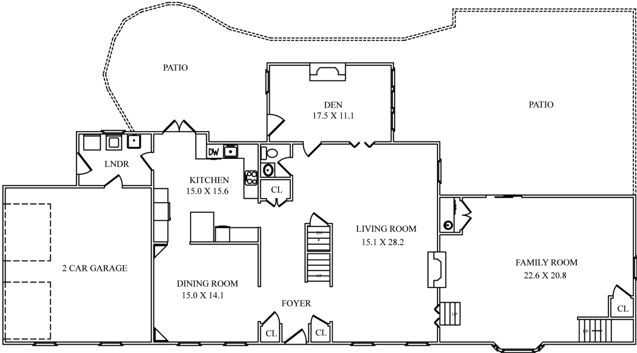
First Floor
