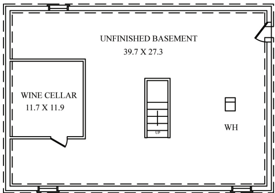
Lower Level
